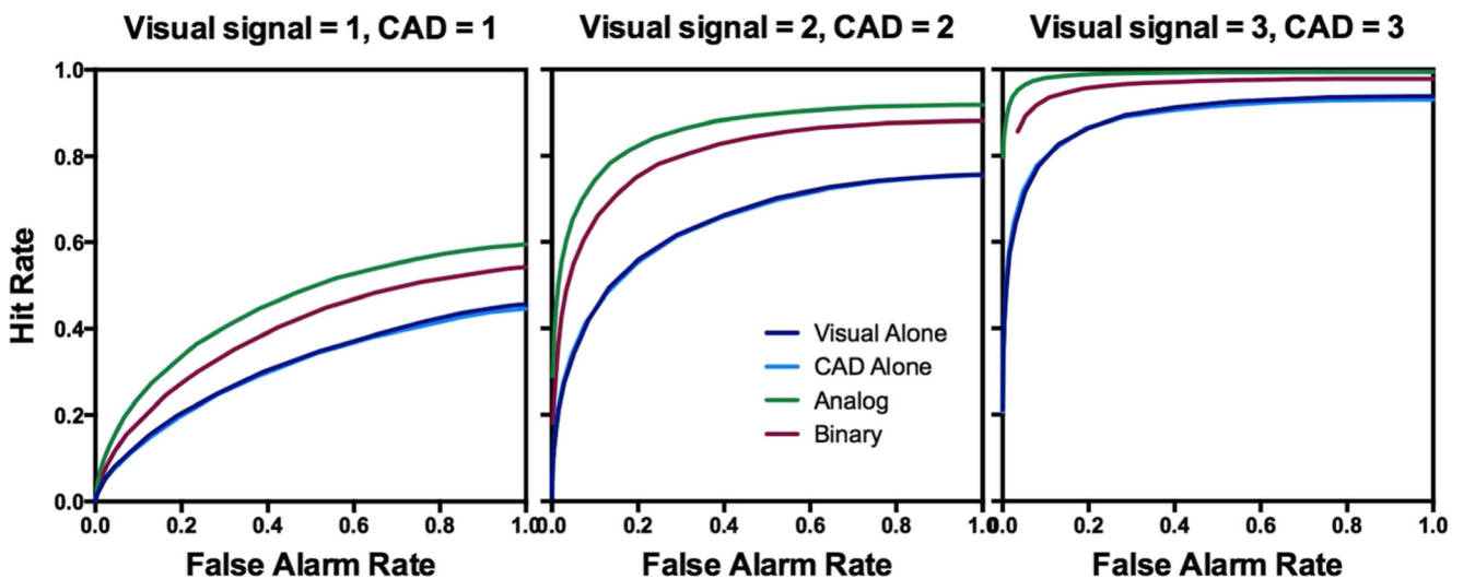
Fig. 4 ROC curves comparing simulations of visual, CAD, analog, and binary conditions over a range of signal strengths
